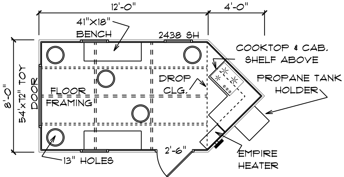
16' "OPEN" MODEL (SIDE ENTRY W/ TOY DOOR)
